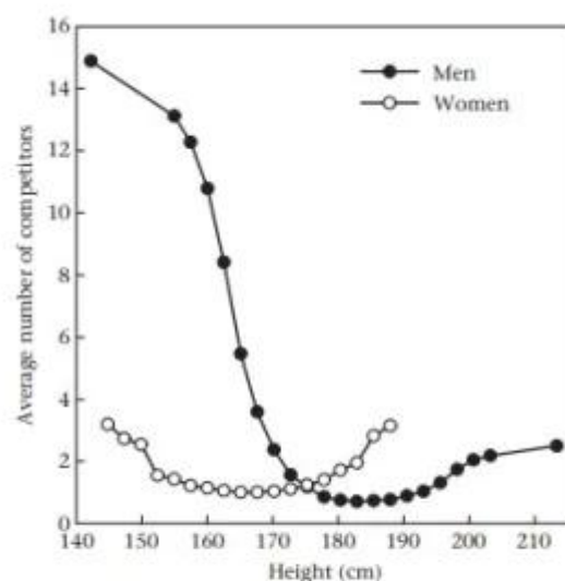
Figure 2. The number of competitors in the speed-date population for men and women in relation to their height. High values indicate that the number of individuals of a given height is high relative to the number of opposite-sex individuals for whom that height falls within the acceptable height range. See text and Tables A3 and A4 for further information.
